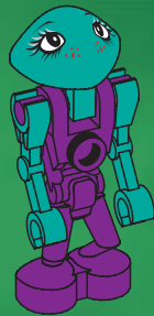
CASSIOPEIA
