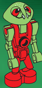
ARCTURES
